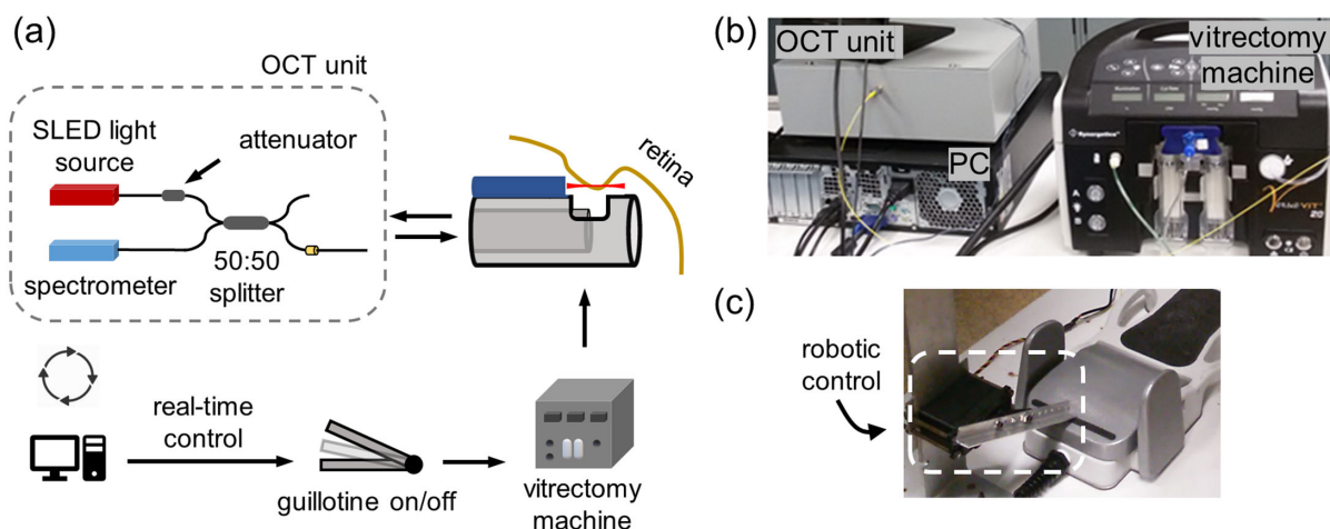
Figure 2. The smart vitrectomy system. (a) Schematic representation of the OCT unit and overview of the injury prevention mechanism. Images of the experimental setup, including (b) the OCT unit, the personal computer (PC), the vitrectomy machine, and (c) the robotic mechanism (i.e., servomotor and metallic beam) used to control the pedal.
